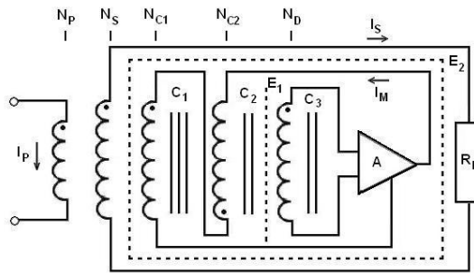
Fig. 2. Electronically-compensated current comparator
